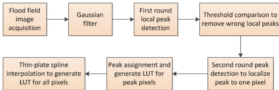
Fig 3. The 2D position calibration flow for the gamma imaging detectors.
