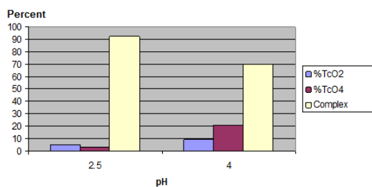
Figure 4. Effect of pH on ^{99m}\text{Tc} -ciprofloxacin radiolabeling yield.
