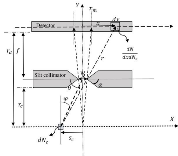
Fig 1. Geometric description of physical parameters for the KE collimator and pixelated detector.
