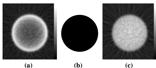
Figure 3. Illustration of reconstruction artifact resulting from lack of attenuation correction for uniform distribution of activity in a cylindrical phantom. (a) Reconstructed image without attenuation correction. (b) Uniform attenuation map at 511 keV. (c) Same slice as (a) after applying attenuation correction. Reprinted with permission from ref. [20].
