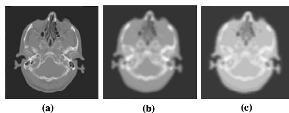
Figure 5. (a) Original CT image acquired at 120 kVp with matrix size 512 \times 512 ; (b) the slice in (a) after down-sampling to 128 \times 128 and Gaussian smoothing with \text{FWHM}=6 mm. (c) Attenuation map of the slice in (b) at 511 keV converted using a bi-linear calibration curve.
