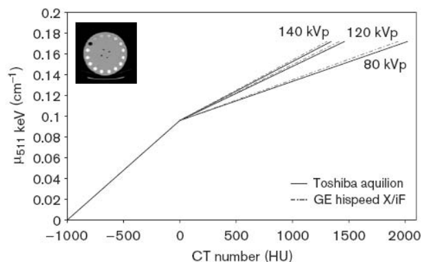
Figure 13. Calculated bi-linear calibration curves for conversion of CT numbers (HU) into linear attenuation coefficients at 511 keV at different tube voltages for both Aquilion and HiSpeed X/iF CT scanners. Reprint with permission from ref. [57].
